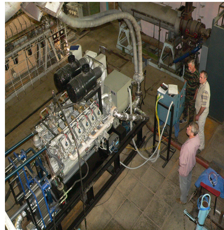
Heat and power plant on the base of gas engine for using gaseous reaction products
